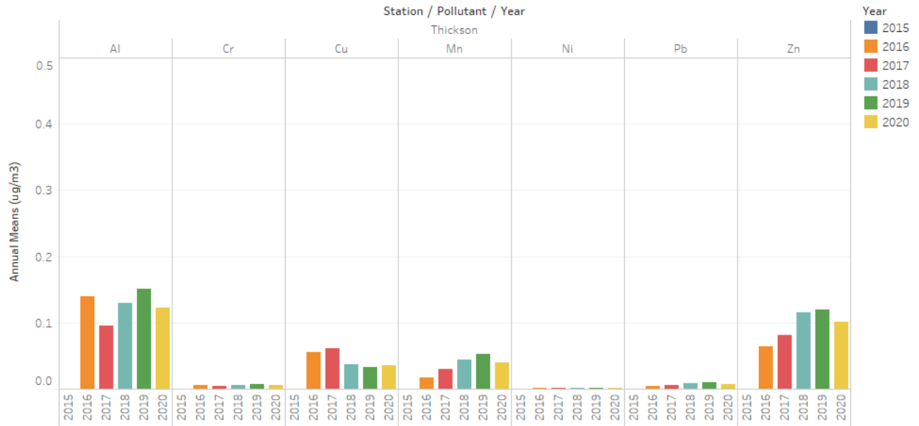
Annual Means for Selected Metals at Gerdau Ameristeel at Thickson Station
