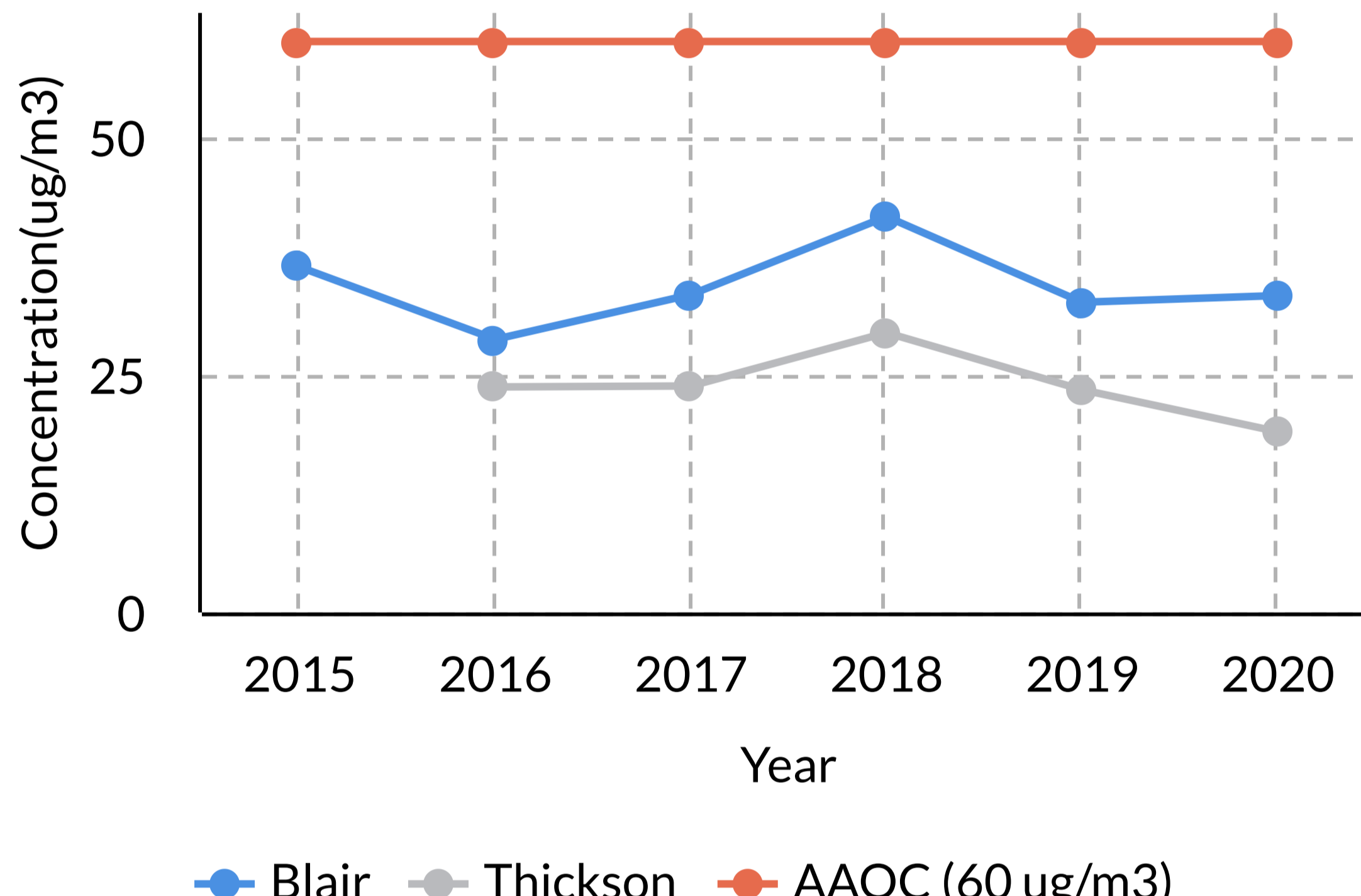
Yearly BaP Levels
