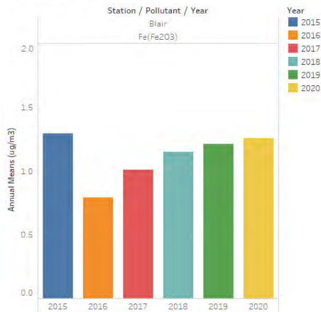
Annual Means for Iron at Gerdau Ameristeel at Blair Station
