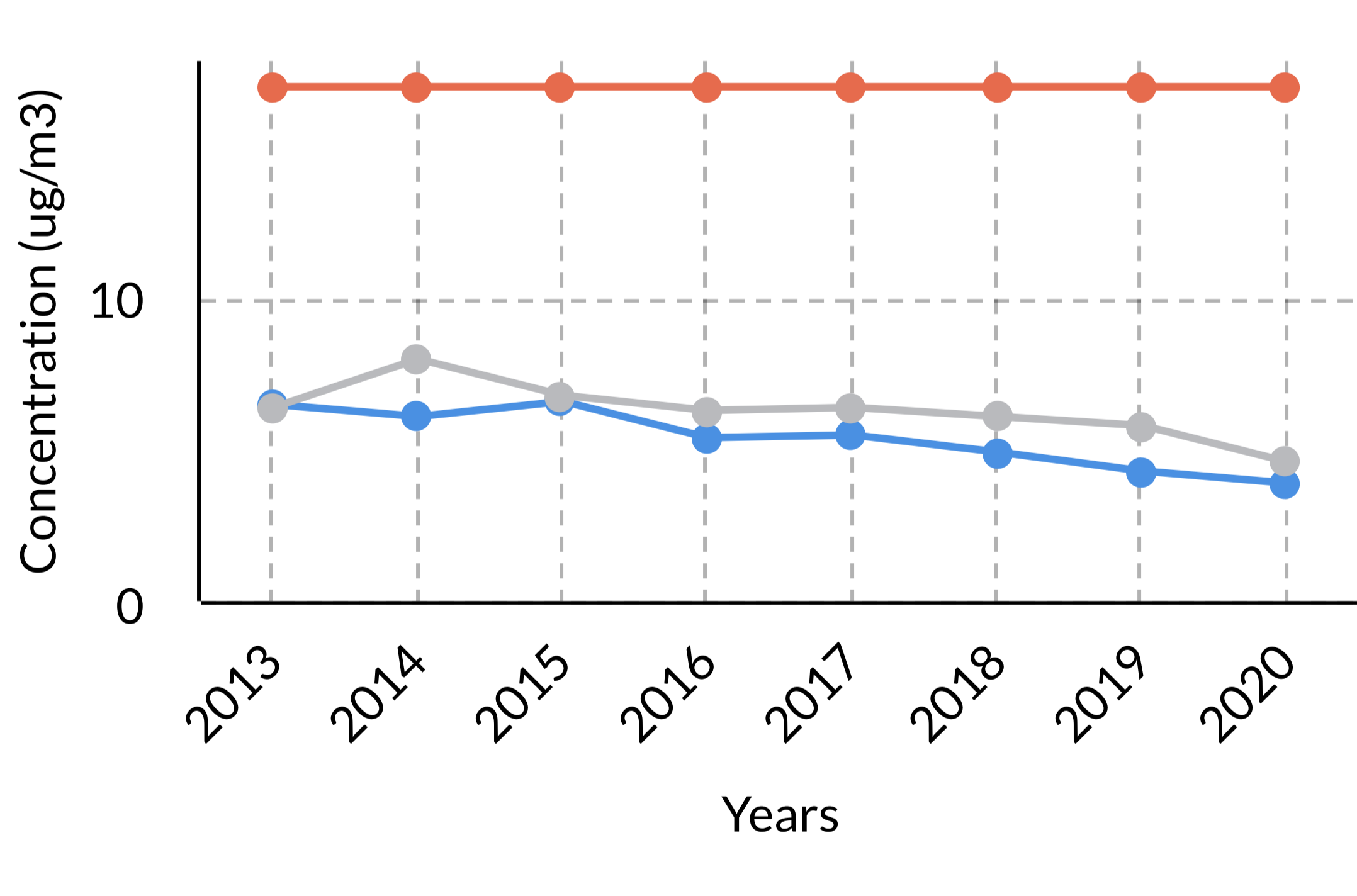
Yearly NO 2 Levels
