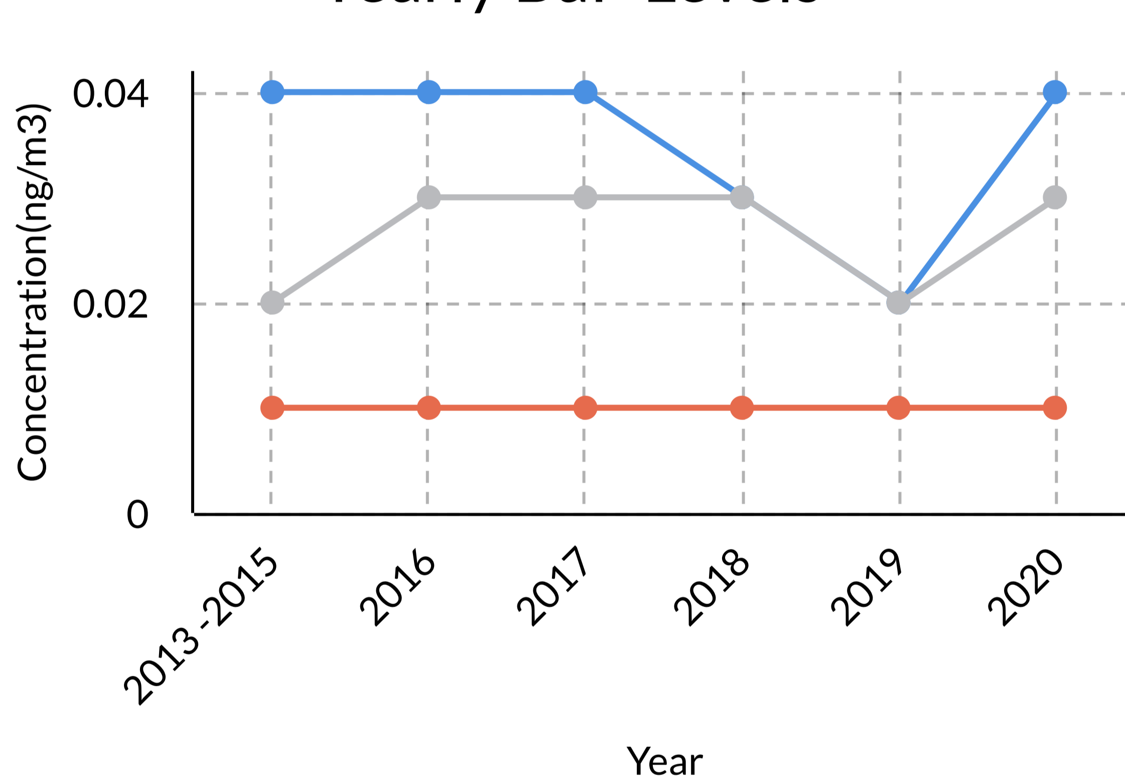
Yearly BaP Levels
