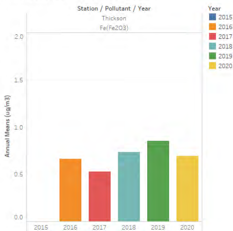
Annual Means for Iron at Gerdau Ameristeel at Thickson Station
