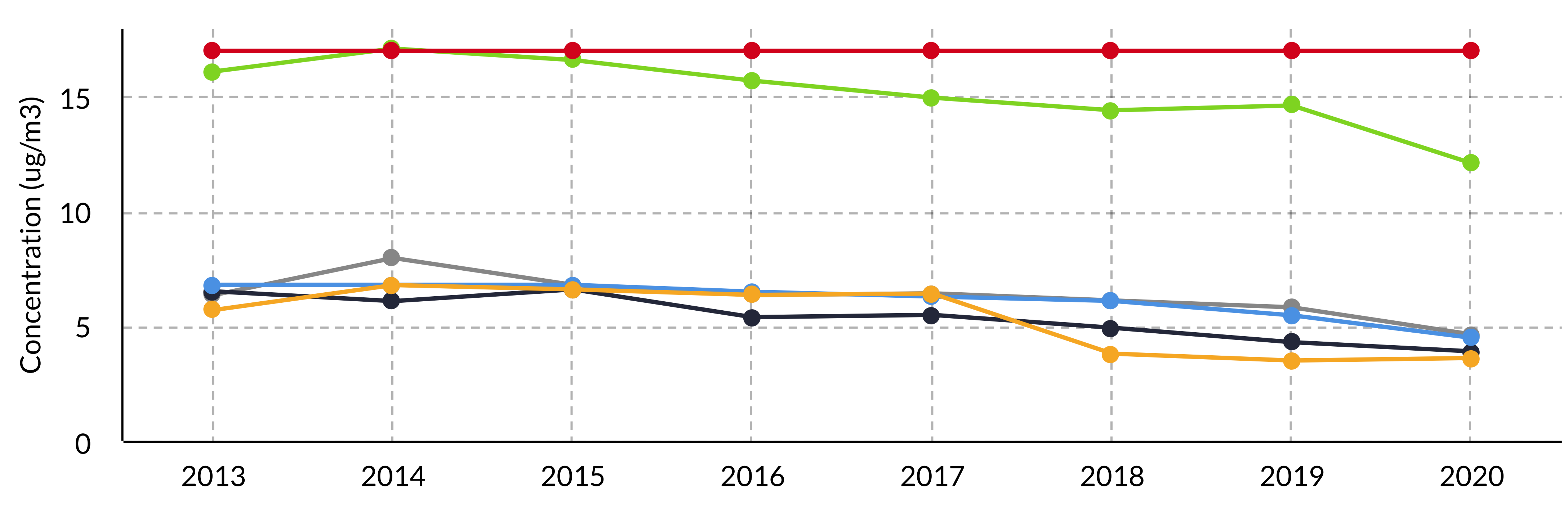
Yearly NO 2 Levels at Multiple Stations
