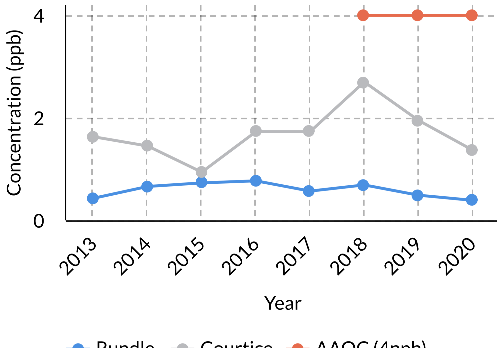
Yearly SO 2 Levels
