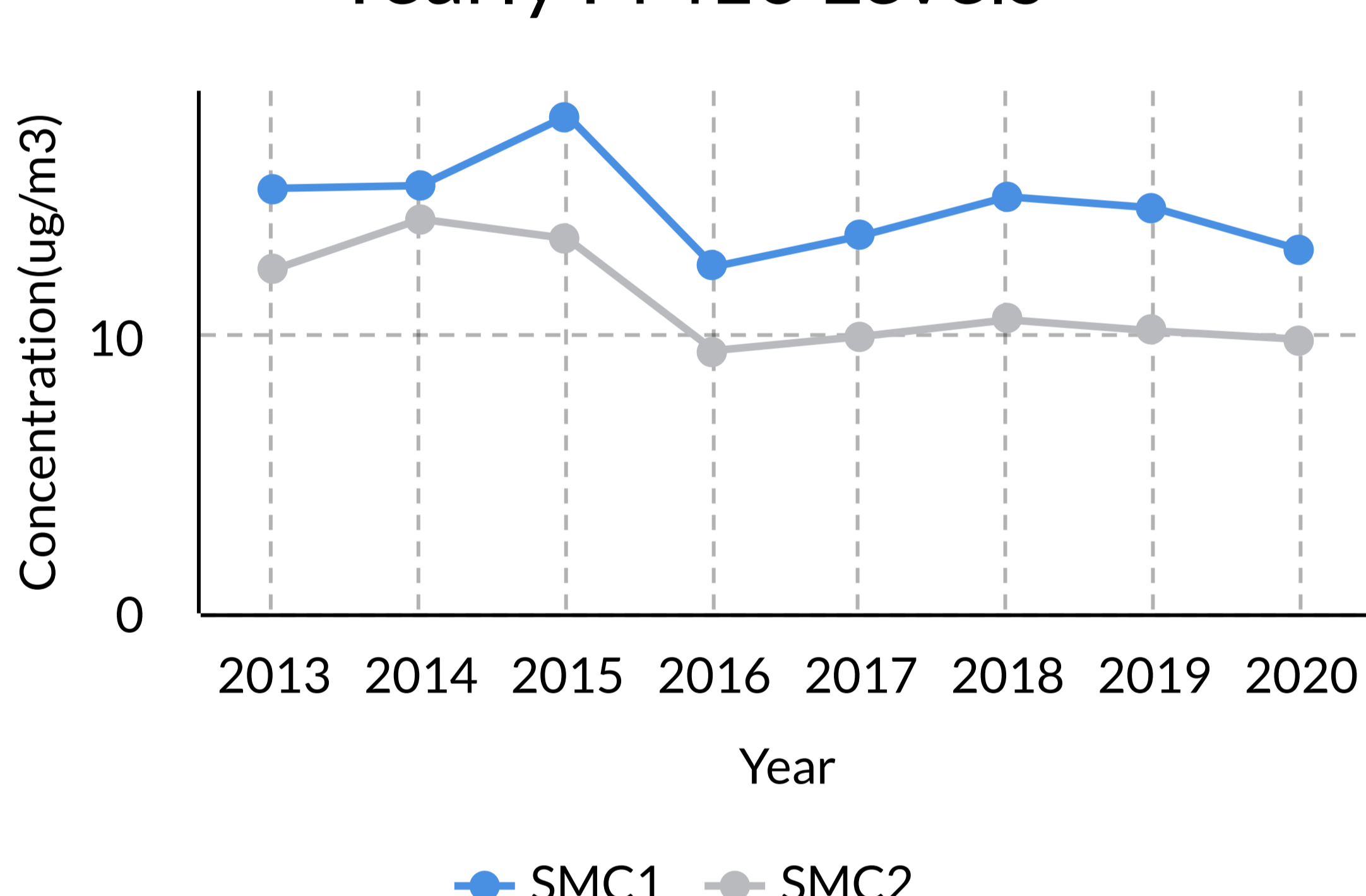
Yearly PM 10 Levels
