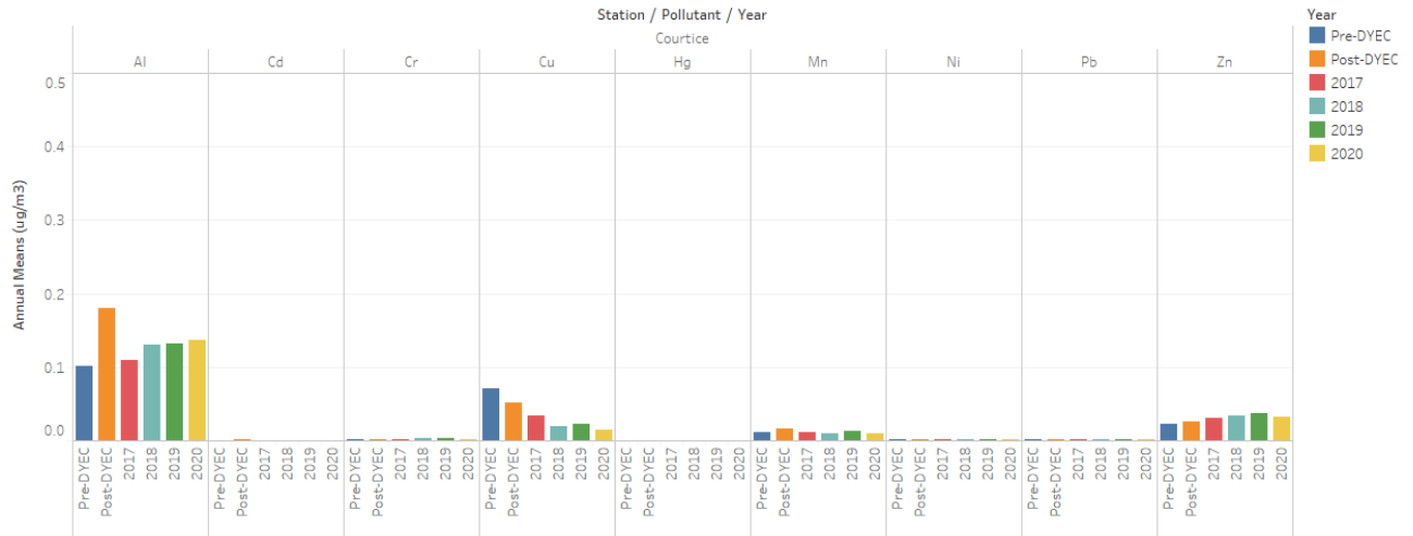
Annual Means for Selected Metals at DYEC at Courtice Station
