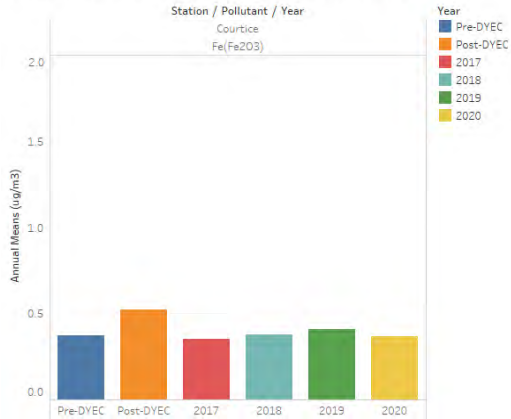
Annual Means for Iron at DYEC at Courtice Station
