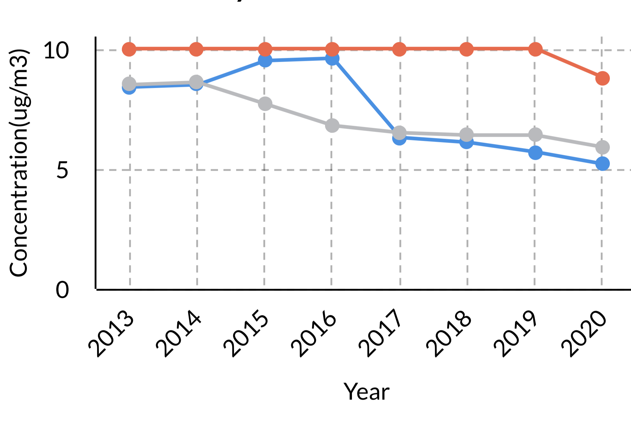
Yearly PM 2.5 Levels
