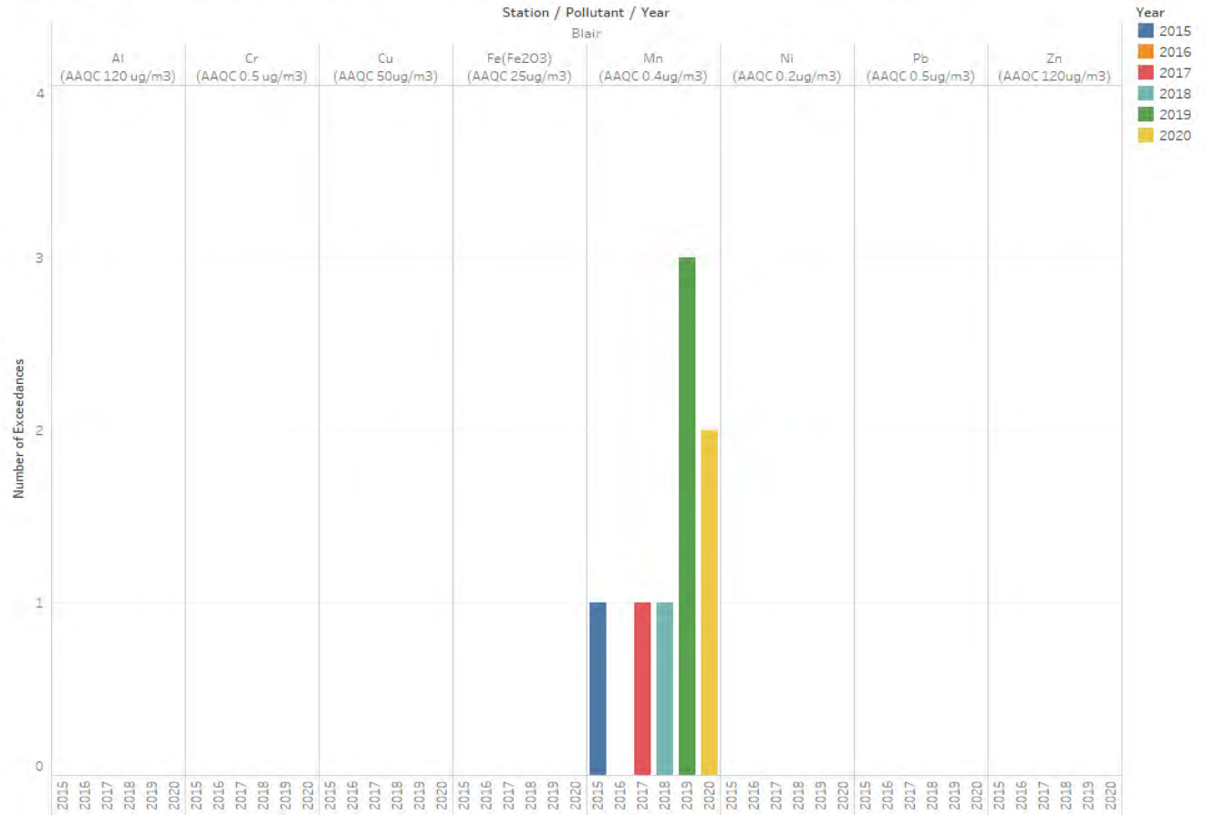
No. of 24-Hour AAQC Exceedances for Selected Metals at Gerdau Ameristeel at Blair Station
