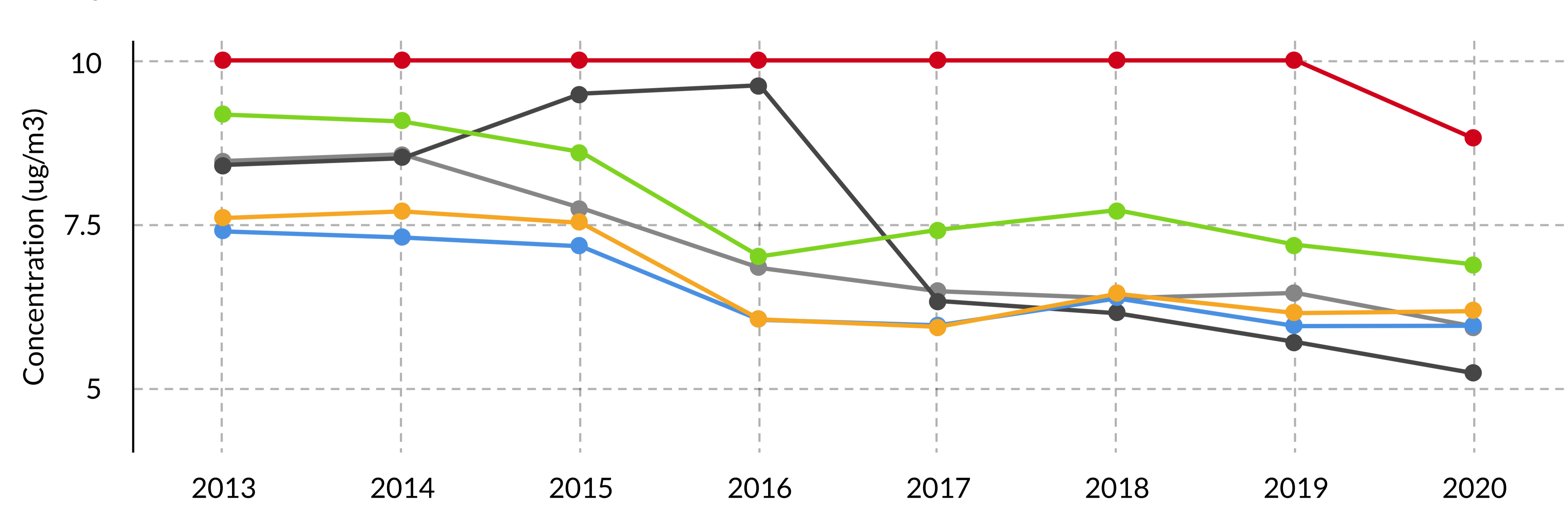
Yearly PM 2.5 Levels at Multiple Stations
