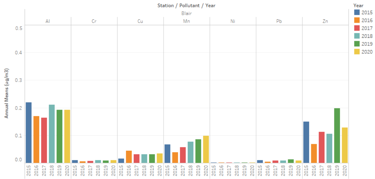
Annual Means for Selected Metals at Gerdau Ameristeel at Blair Station
