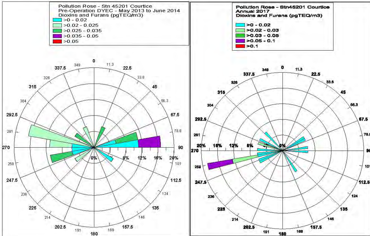
Figure C5 Dioxins and Furans 24-hour Average Pollution Roses – DYEC Monitoring Program - Courtice
